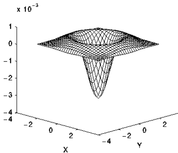
Figure 1: The 2-D Laplacian of Gaussian (LoG) function. The x and y axes are marked in standard deviations ( \sigma ).
