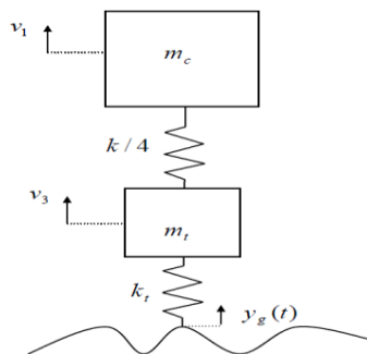
Figure 1.4. A quarter car suspension model (Source: Gobbi and Mastinug)
