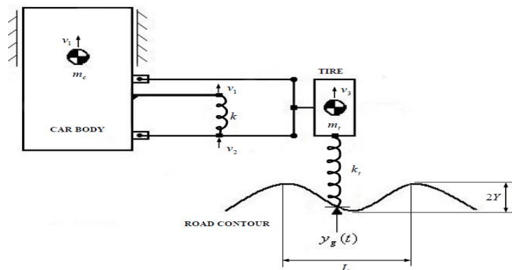
Figure 1.4. Simple model of the suspension system
