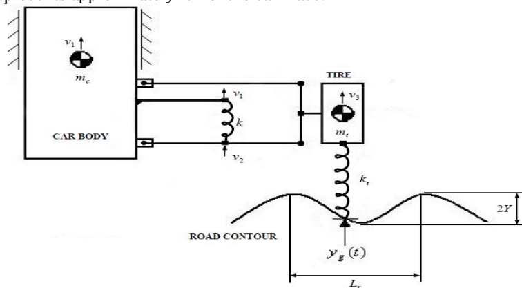
Figure 1.3. Simple model of the suspension system
