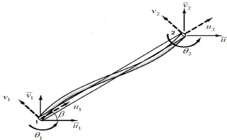
Figure 1.1. Plane frame element (Source: Belegundu and Chandrupatla 1997)
