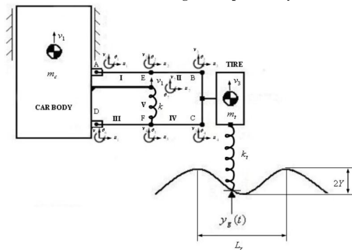
Figure 1.5. Finite element model of the suspension system
