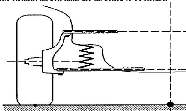
Figure 1.2 A quarter car with the double wishbone suspension (Source: Gillespie 1992)
