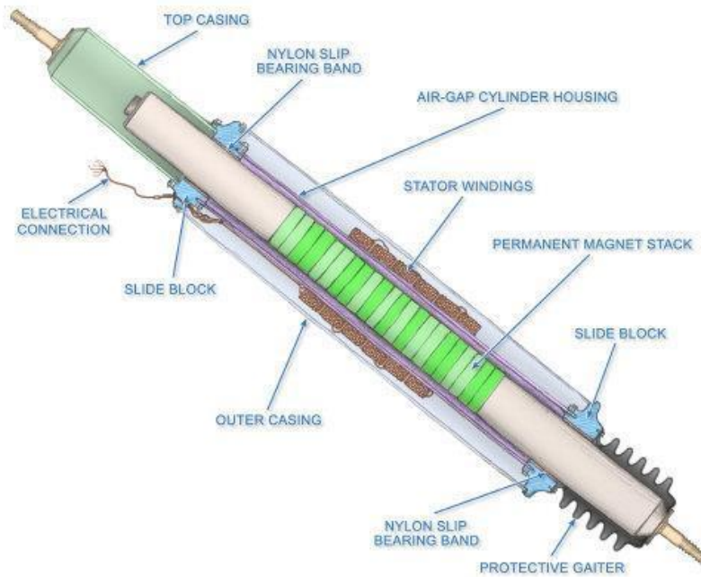
Figure 3.1 : Example of Power-Generating Shock Absorber
