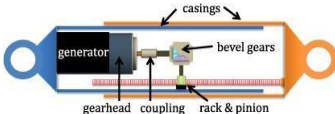
Figure 3.5: Traditional design of a rack-pinion based power generating shock absorber
