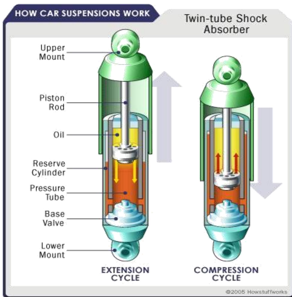
Figure 2.3: Twin Tube Shock Absorber
