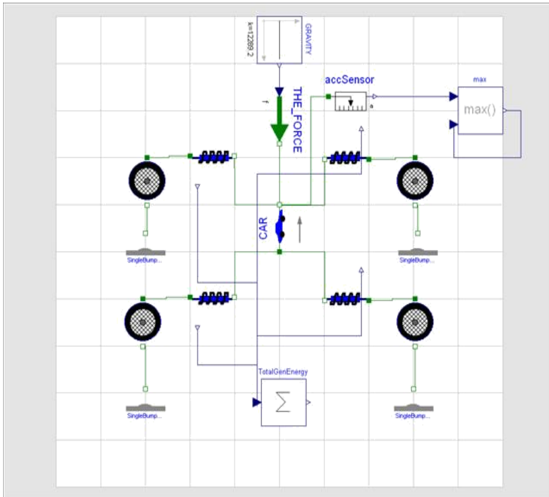
Figure 3.3: Model of entire car including four tires and entire suspension.
