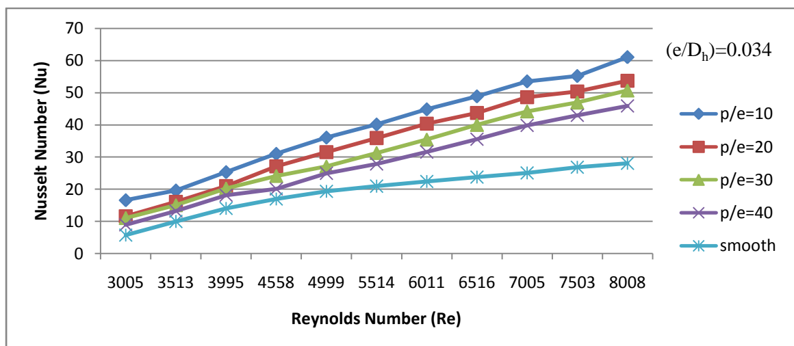
Fig.4. Variation of Nusselt number with Reynolds number for different values of (p/e) and for a fixed value of (e/D h ) for Single arc geometry.
