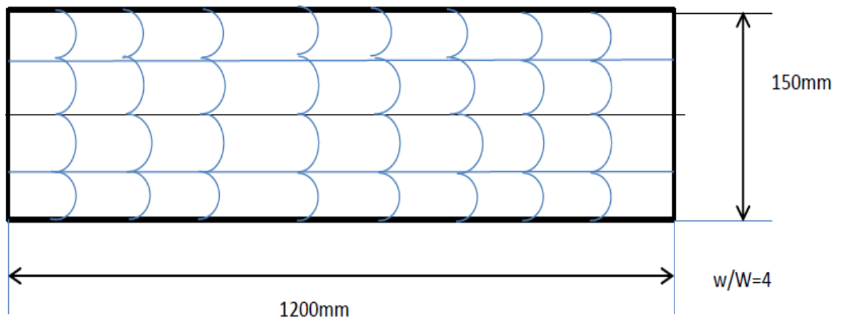
Figure 2. Four arc shaped artificial roughness( w/W=2 )
