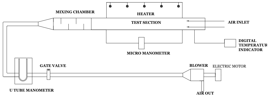
Figure 3. Experimental setup
