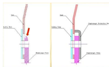
Figure 6: Insertion of diaphragm protection sheets
