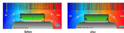
Figure 5: Before and After sealing
