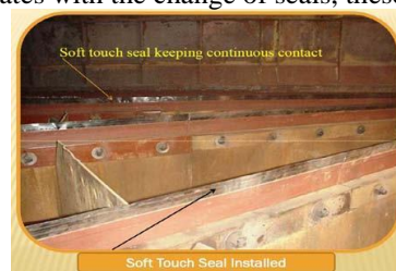
Figure 4: Installation of soft touch seal
