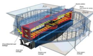
Figure 1: 3-D View of Ljungstrom Air pre-heater
