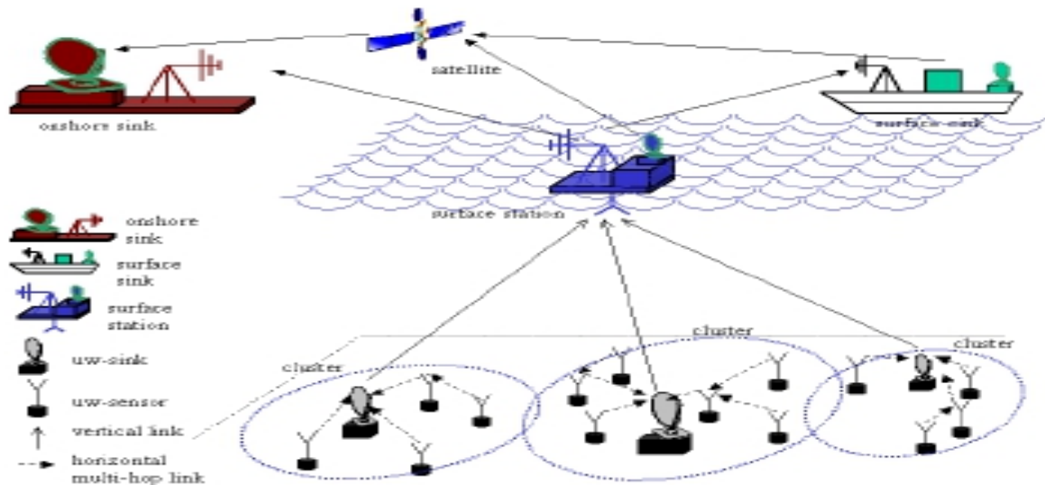
Fig. 1. Architecture for 2D Underwater Sensor Networks.
