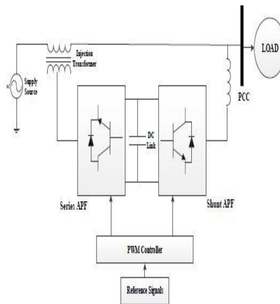
Fig. 5: UPQC with controller arrangement
