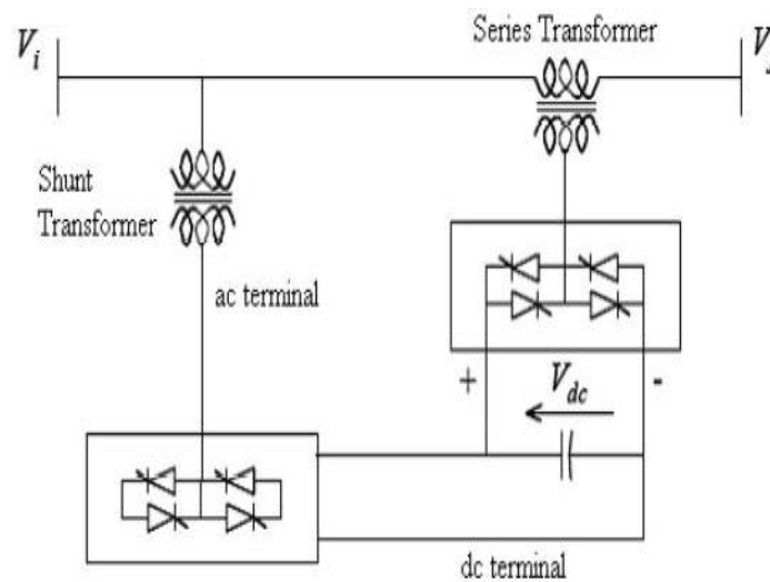
Fig. 4 Configuration of UPFC
