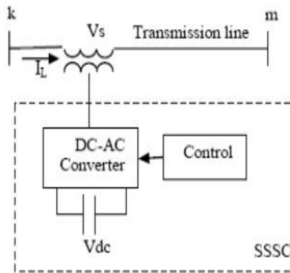
Fig. 3 Simplified diagram of a SSSC
