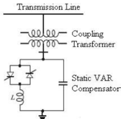
Fig No.1 Configuration of SVC
