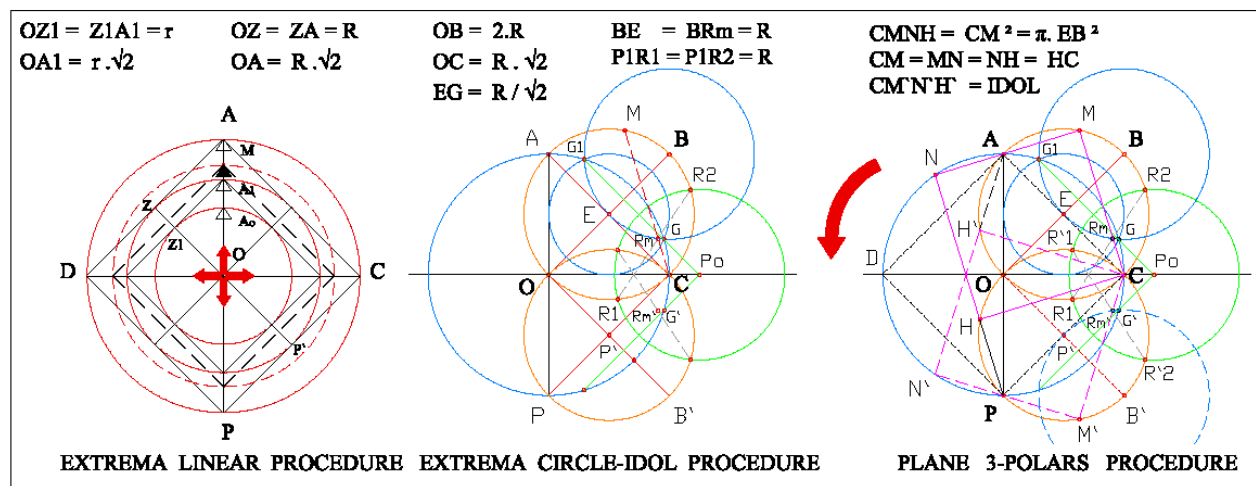
Figure 48 : The Extrema Linear Expanding Squares , interchange on Extrema Plane Rotating Squares through the four Conjugate circles of monad AC to square CMNH equal to that of the circle.
