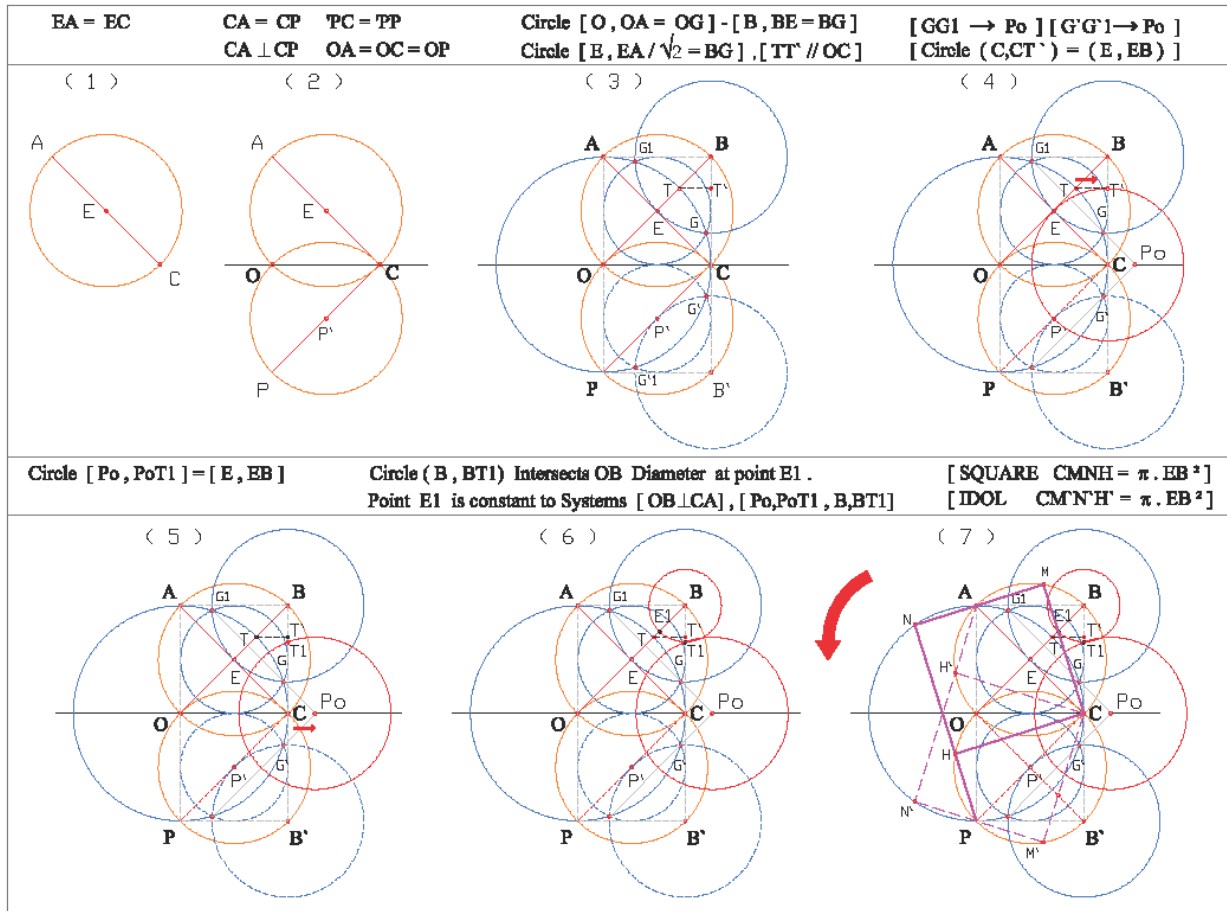
F.50 → The Squaring of the circle using Extrema-Kinematic Method.
