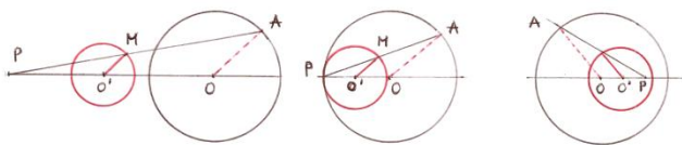
Figure 9. A point and a circle – (5.2)
