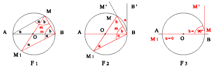
Figure 13. All angles on a diameter of a circle are 90^\circ . (5.5.2)
