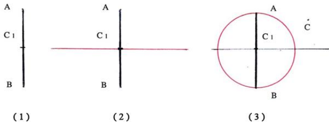
F.36. A Segment , the middle , and the Circle on Segment .
