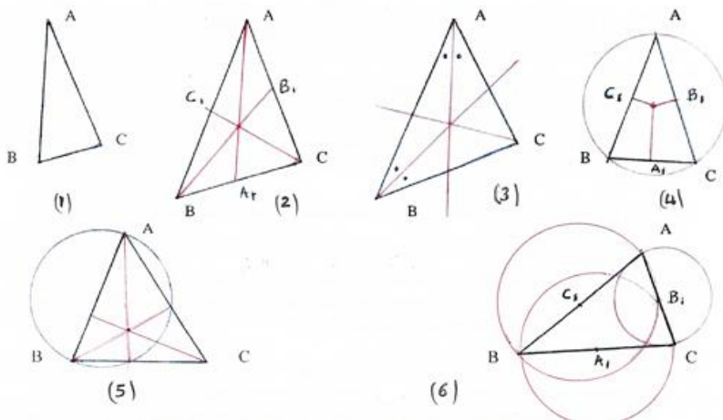
F.39. The different properties on any triangle ABC .
