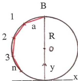
F.40. The n roots of R = OB
