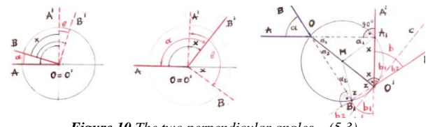
Figure 10. The two perpendicular angles – (5.3)
