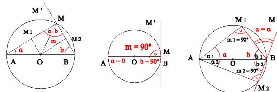
Figure 11. The two perpendicular supplementary angles in Extrema presentation – (5.4)
