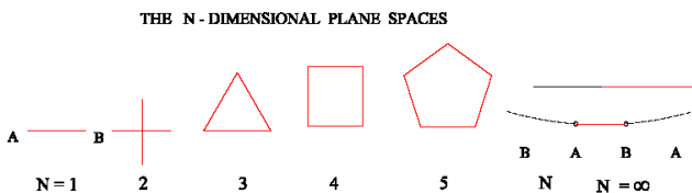
Figure 4. The Increasing Space Layers – (4)
