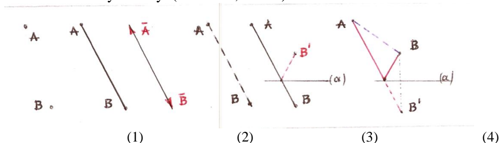
Figure 23 . A point and a line of any direction :
