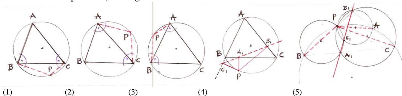
Figure25. The position of a point P and any circumcircle on any triangle ABC :
