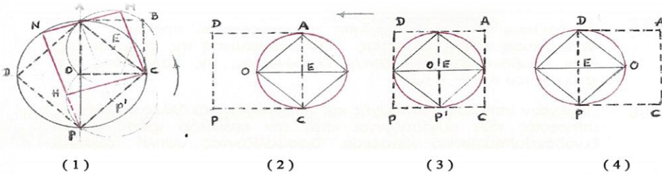
F.44. The Inscribed square ACPD on O,OA Circle of Rotating Resemblance ratio 2 .
