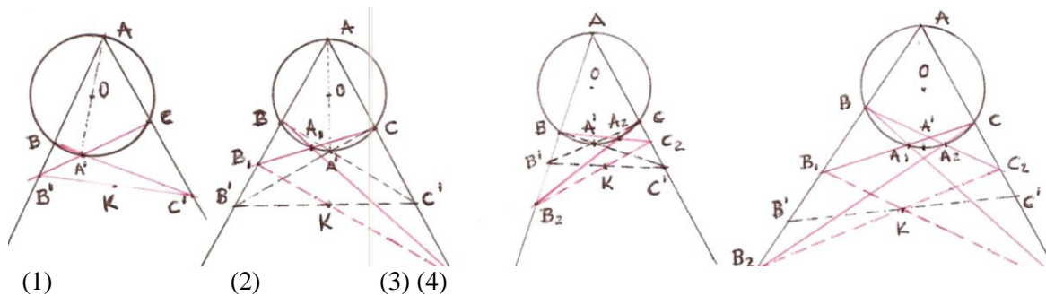
Figure 27. Extrema points on any circumcircle of triangle ABC :
