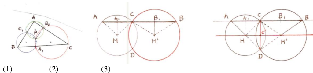
Figure 22 . A point M and any line directional to AB :
