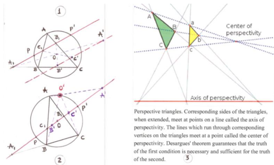
Figure 26. The two Perspective triangles ABC – abc :
