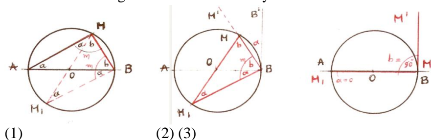
Figure20 . A point M on any circle of diameter the monad AB :
