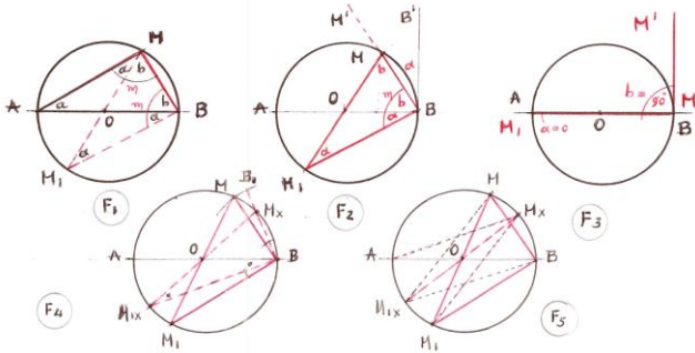
Figure 14. An angle on any circle - (5.5.3)
