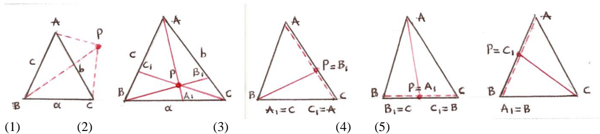
Figure 24 . The position of a point P and any triangle ABC :
