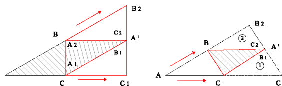
Figure 8. The Rational figures – (5.1)
