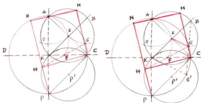
F.41. The moving Square(CMNH=Space)and Anti-square (Idle)on a circle .
