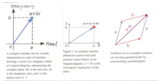
Figure 15. The Quaternion of Spaces – (7)
