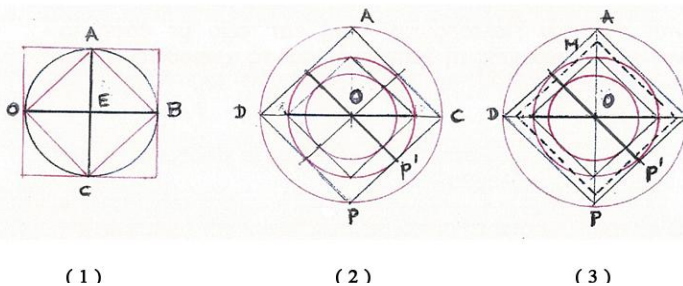
F.45. The Circumscribed and Inscribed Square on a circle of Drawing Resemblance ratio 2 .
