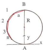
Figure 16. The Unit circle of the Polygons - (7) y_B = [2 \cdot R]
