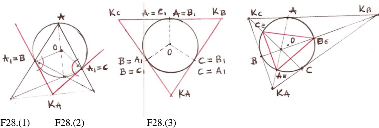
Figure 28. Concurrency points in and out of any circumcircle of triangle ABC :
