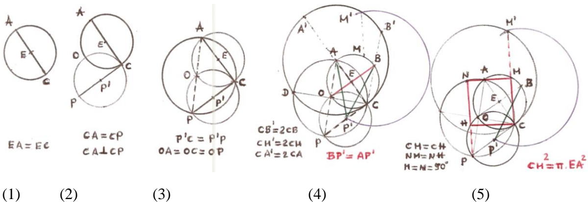
F.47. The circumscribed Circle and Square on a circle.
