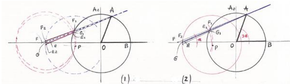
F.34. The Trisection method of any angle \angle AOB
