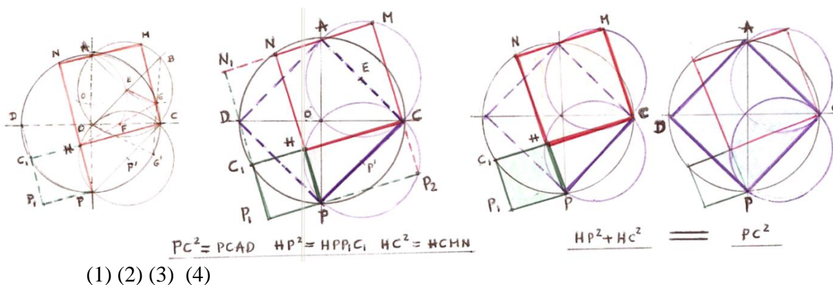
F.43. The moving Squares (CMNH = Space) and Supplementary anti-squares (PHC1P1=Idle) on circle .
