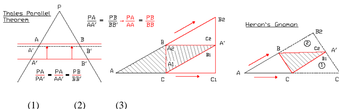
Figure 19 . The Extrema in Thales theorem and Rational Figures – (7)
