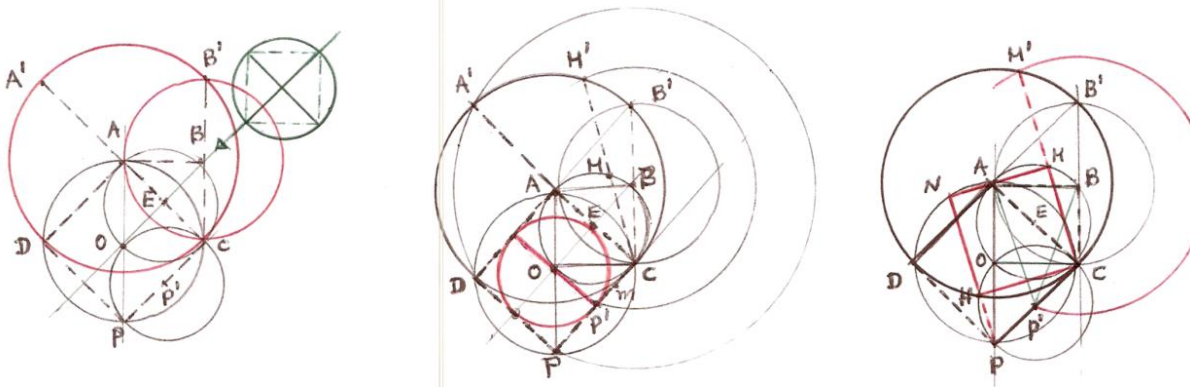
(1) (2) (3) F.46. The Geometrical Machine making all Squares on a circle .
