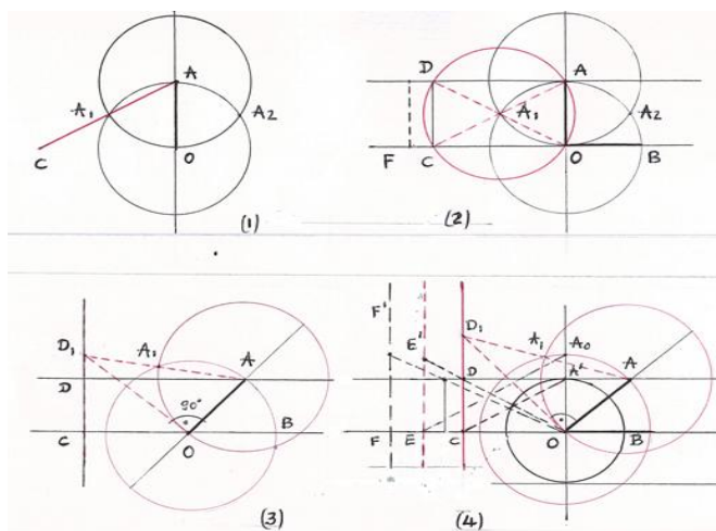
F.32. The proposed Contemporary Trisection method .
