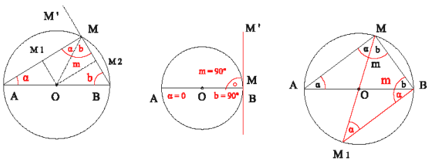
Figure 12. An angle on a circle with Extrema cases - (5.5.1)
