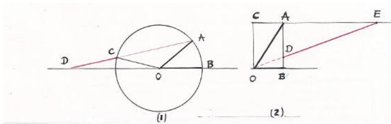
F.31. Archimedes (1) and the Pappus (2) Trisection method .
