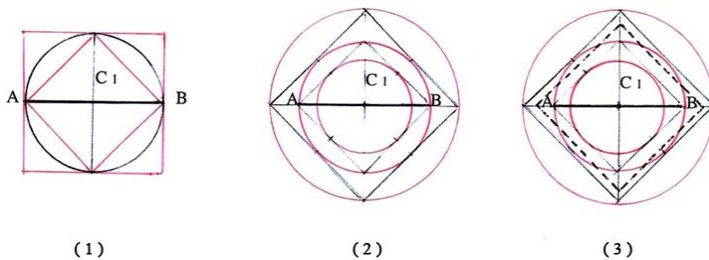
F.37. The circumscribed Circle and Square on a circle .
