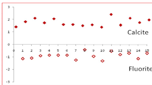
Fig. 7: Saturation index of Calcite ( \text{CaCO}_3 ) and Fluorite ( \text{CaF}_2 ) represents oversaturated and under saturated in groundwater samples of the study area
