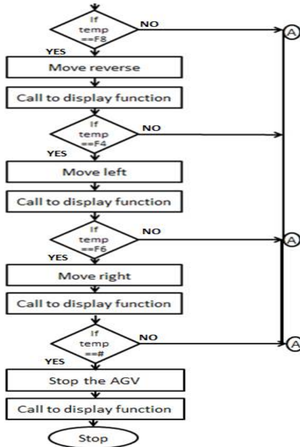
Fig6. Flowchart for Robot's Movement Control
