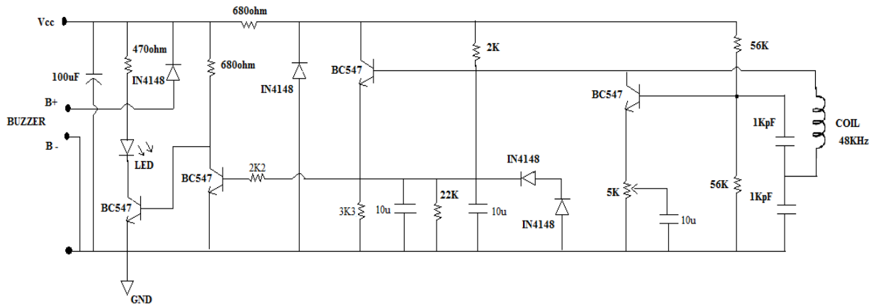
Fig5. Circuit Diagram of Metal Detector
