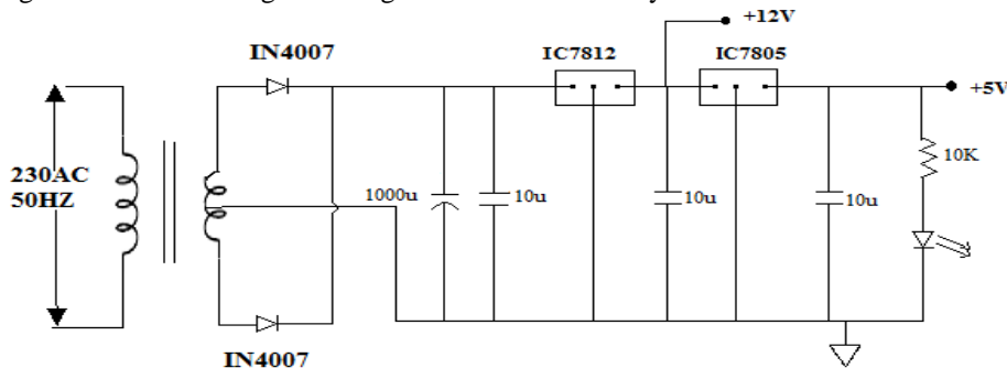
Fig2. Circuit diagram of power supply unit
