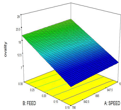
Figure 5. Ovality from regression modeling
