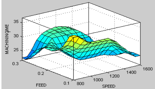
Figure 18 Machining time from FIS
