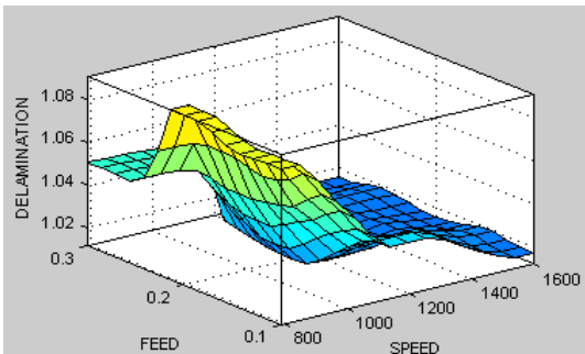
Figure 14. Delamination from FIS
