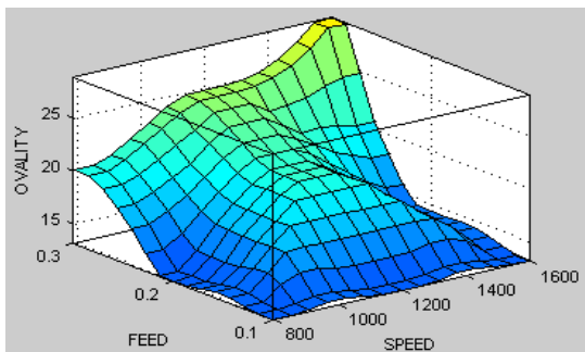
Figure 20. Ovality from FIS
