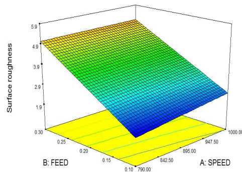
Figure 9 Surface roughness from regression modeling
