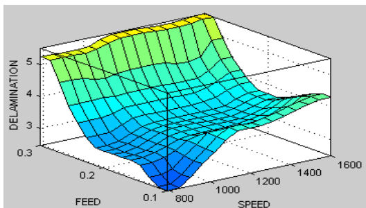
Figure 22. Delamination from FIS
