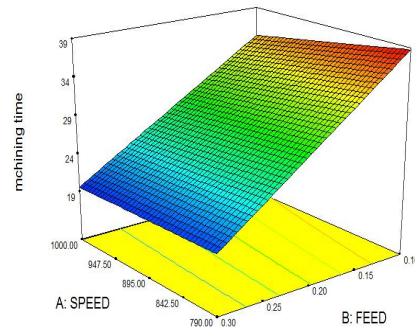
Figure 19. Machining time from regression modeling
