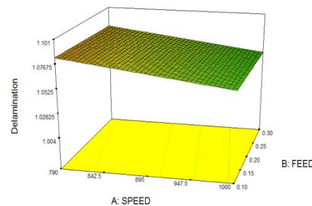
Figure 7. Delamination from regression modeling
