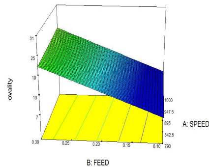
Figure 21. ovality from regression modeling.
