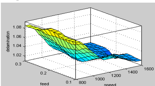
Figure 6. Delamination from FIS
