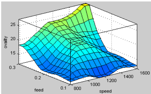
Figure 4. Ovality from Fuzzy inference system (FIS) model
