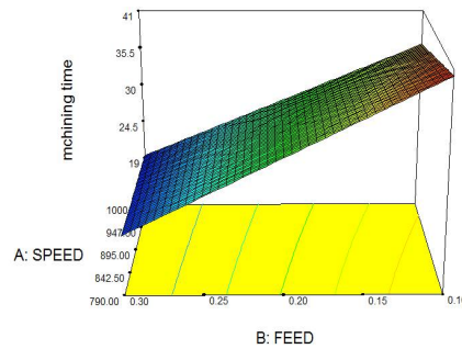
Figure 3. Machining time from regression model
