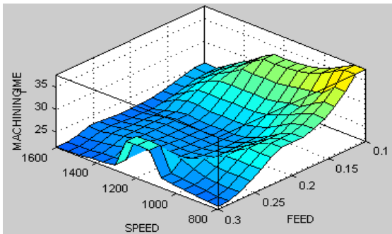
Fig 10 machining time from FIS
