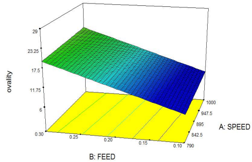
Figure 13. Ovality from regression modeling
