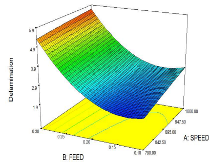
Figure 23. Delamination from regression modeling
