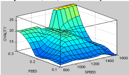
Figure 12 Ovality from FIS
