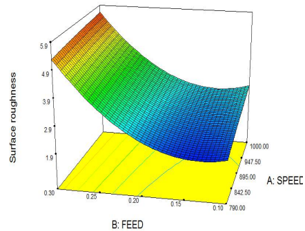
Figure 25. Surface roughness from regression modeling
