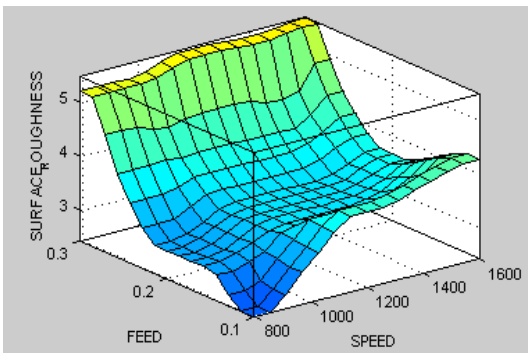
Figure 24. Surface roughness from FIS
