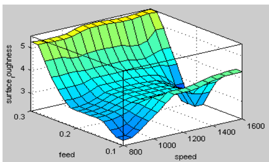
Figure 8. Surface roughness from FIS
