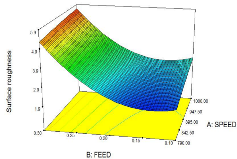
Figure 17. surface roughness from regression modeling
