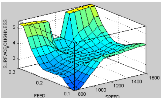
Figure 16. Surface roughness from FIS
