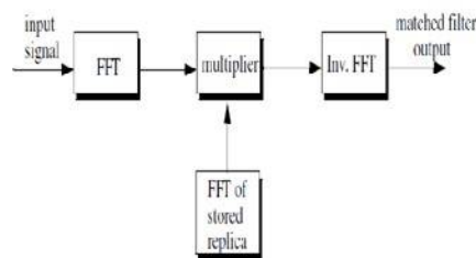
Figure5. Computing the matched filter output using FFT.
