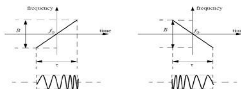
Figure 4. LFM Up chirp and Down chirp signal
