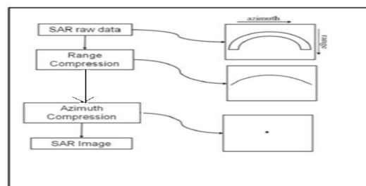
Figure3. Range compression flow graph Or steps.
