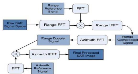
Figure2. Block Diagram of Range Doppler Algorithm.
