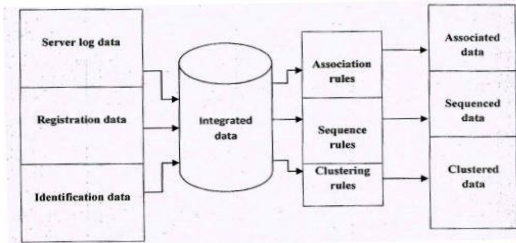
Fig 1: Architecture of Web Mining for online Clothes Shopping.
