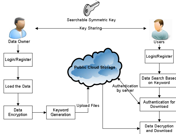
Figure 2: Architecture of ESE framework
