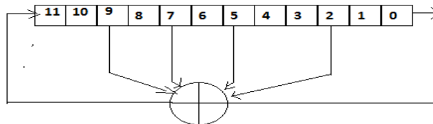
Fig – 3: LFSR
