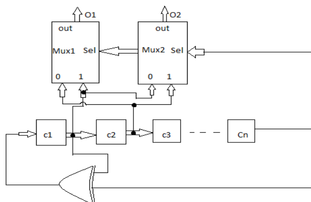
Fig – 8: BIT SWAPPING LFSR
