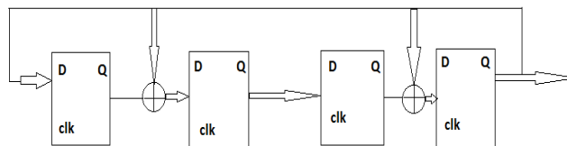
Fig – 6: INTERNAL FEED BACK LFSR
