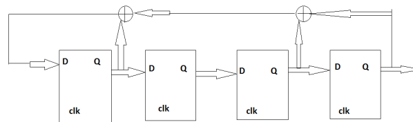
Fig – 4:EXTERNAL FEED BACK LFSR
