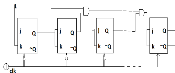
Fig – 5: COUNTER
