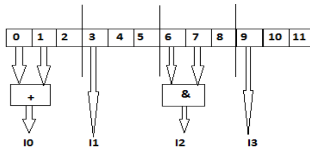
Fig.2. On-chip generation of Input sequence H.
