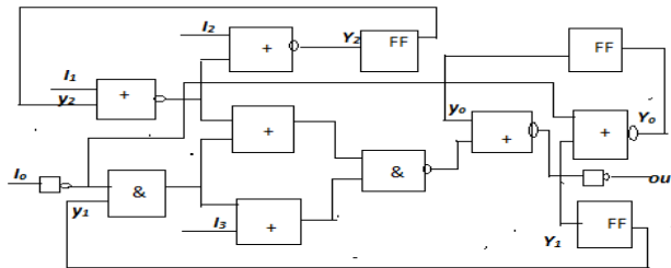
Fig.1.Circuit under test
