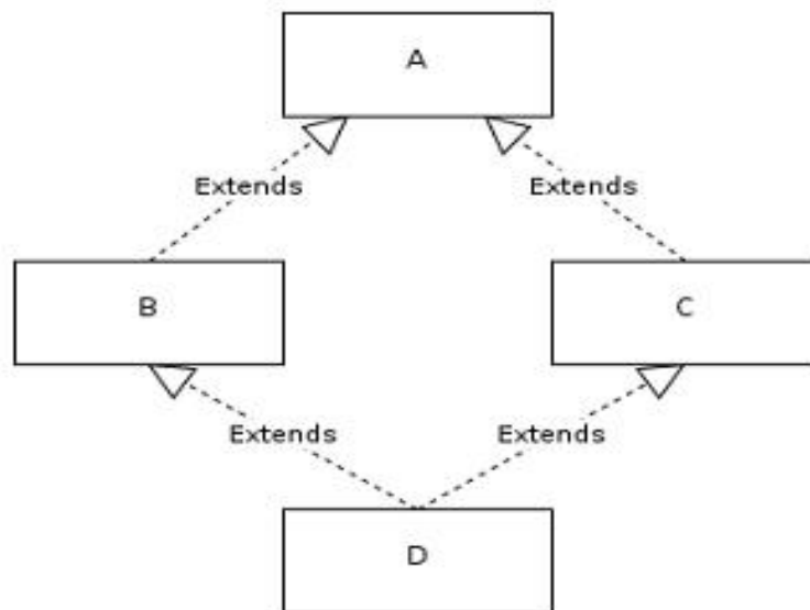
Fig.1 Diamond problem of multiple inheritances
