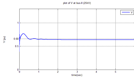
Fig.5 Variation of voltage at PCC without STATCOM
