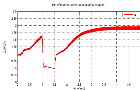
Fig.8 Variation of reactive power generated by STATCOM
