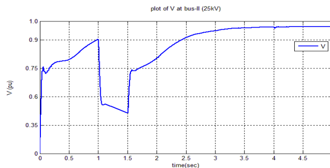
Fig.6 Variation of voltage at PCC with STATCOM
