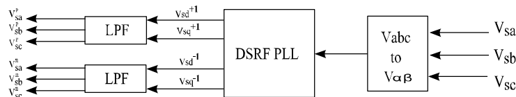
Fig.3 Structure model of the DSRF PLL
