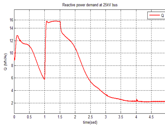
Fig.7 Variation of reactive power demand of wind farm at PCC
