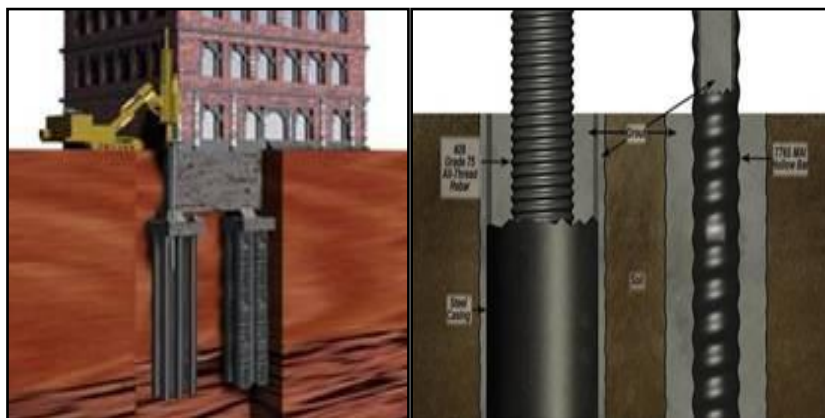
Fig-15 Micro-piles
