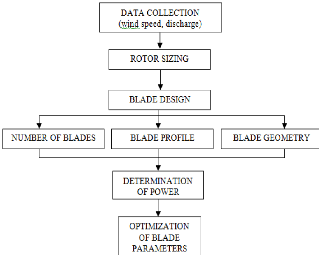
Figure No 6 : Design procedure of small wind turbines [8]
