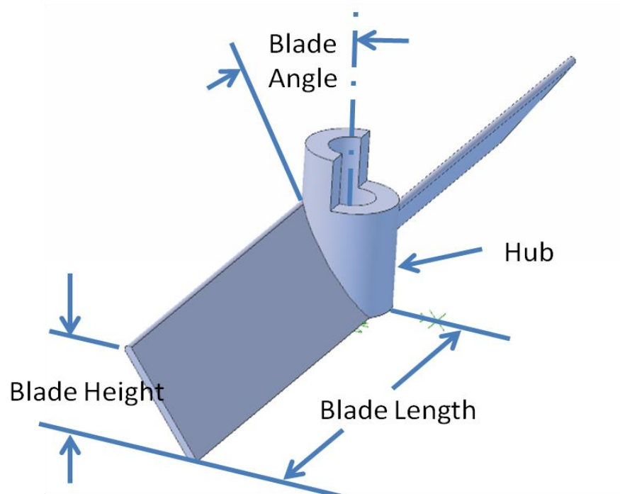
Figure No 8: Optimization of blade parameters [6]
