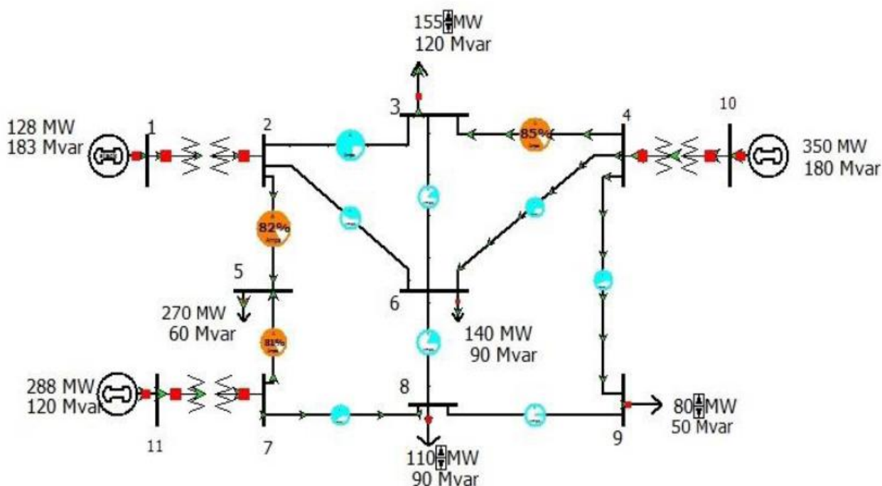
Fig 2 Eleven bus power system
