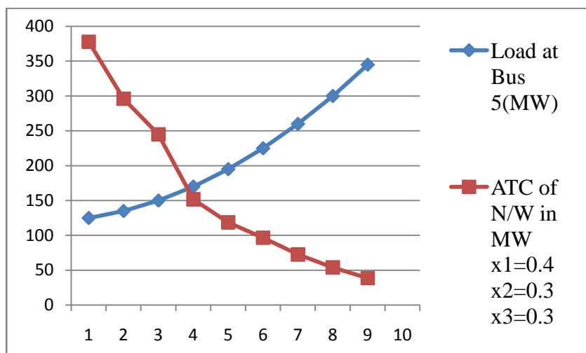
Fig.3 ATC & Load Variation
