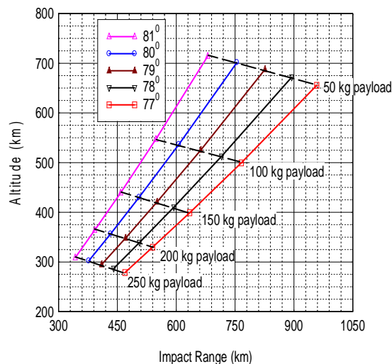
Fig.9. Performance of sounding rocket for various LEA with different payloads
