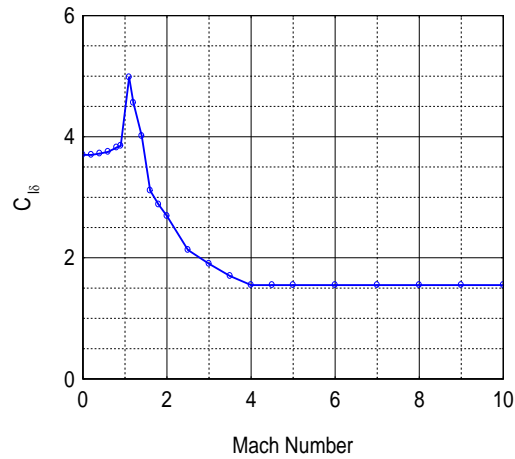
Fig.4. Rolling moment coefficient derivative due to booster fin cant Vs Mach No.
