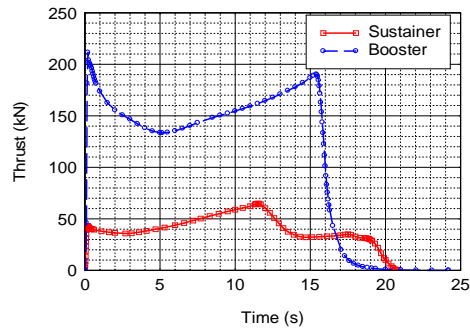
Fig.1. Thrust-Time Profile of the Rocket
