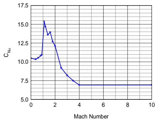
Fig.3. Normal Force Coefficient with respect to Mach No.
