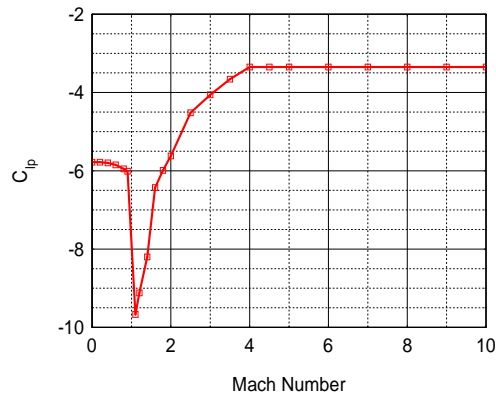
Fig.5. Dynamic Derivative (Roll damping moment coefficient derivative due to rolling velocity) Vs Mach No.
