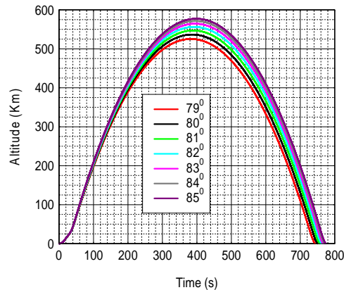
Fig.8. Time Vs. Altitude for various Launch Elevation Angles
