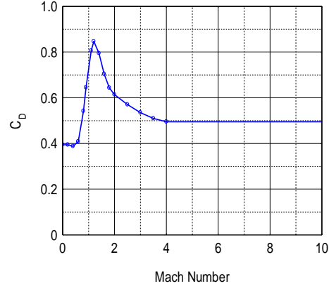
Fig.2. Drag Coefficient with respect to Mach No.
