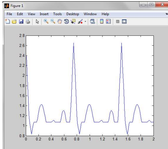
Figure 3.(c)Simulation for Heartbeat Rate 80/Sec
