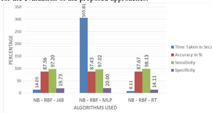
Fig 5. Performance Measures of Three-Staged Classifier with Chi 2
