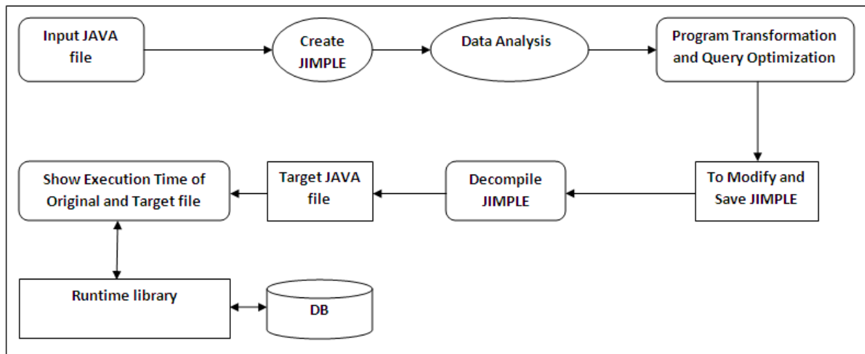
Figure 1- System architecture- Automatic Program Rewriting for Asynchronous and Batched Query Submission
