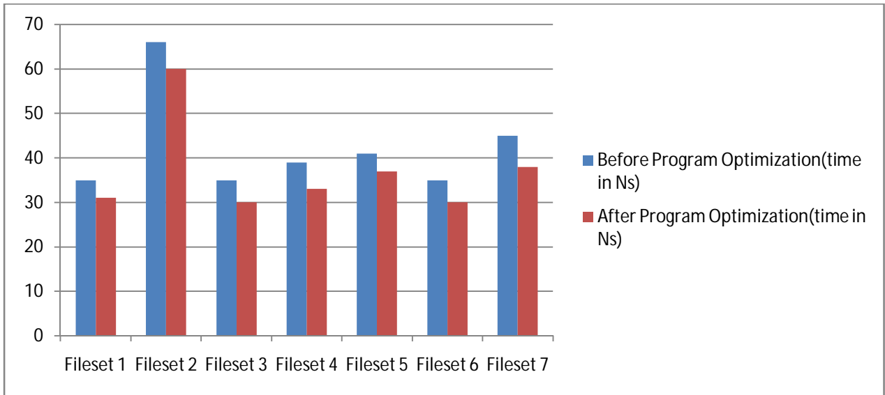
Figure 2- Experiment 1 with execution time for original v/s program optimized files
