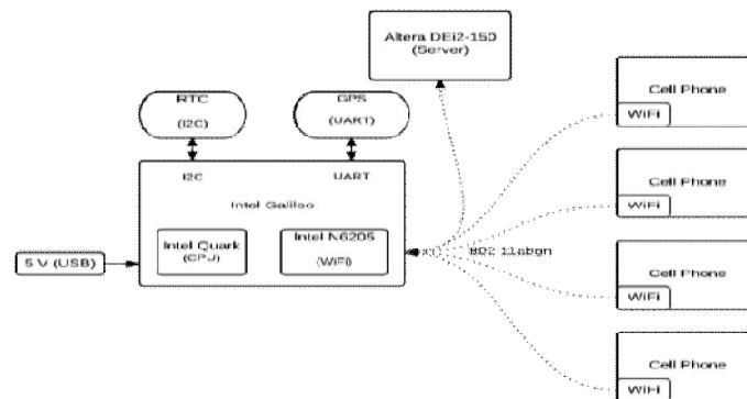
Figure 2. Hardware block diagram.
