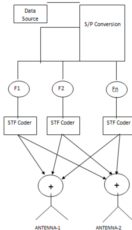
Fig.1. System Model for Separate STF coding rule
