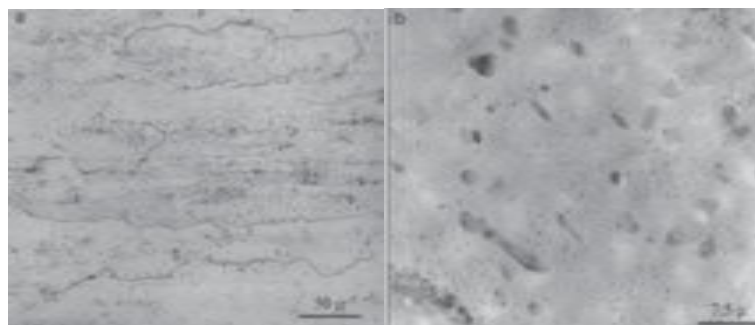
Fig. 1 Microstructure of base metal (a) Optical (b) TEM showing strengthening precipitates
