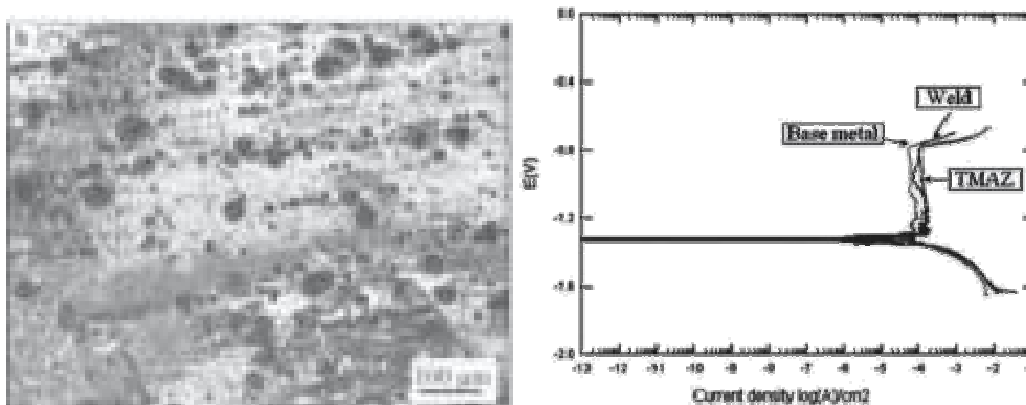
Fig. 5 : Polarization curves of base metal, TMAZ and weld regions in 3.5% NaCl solution
