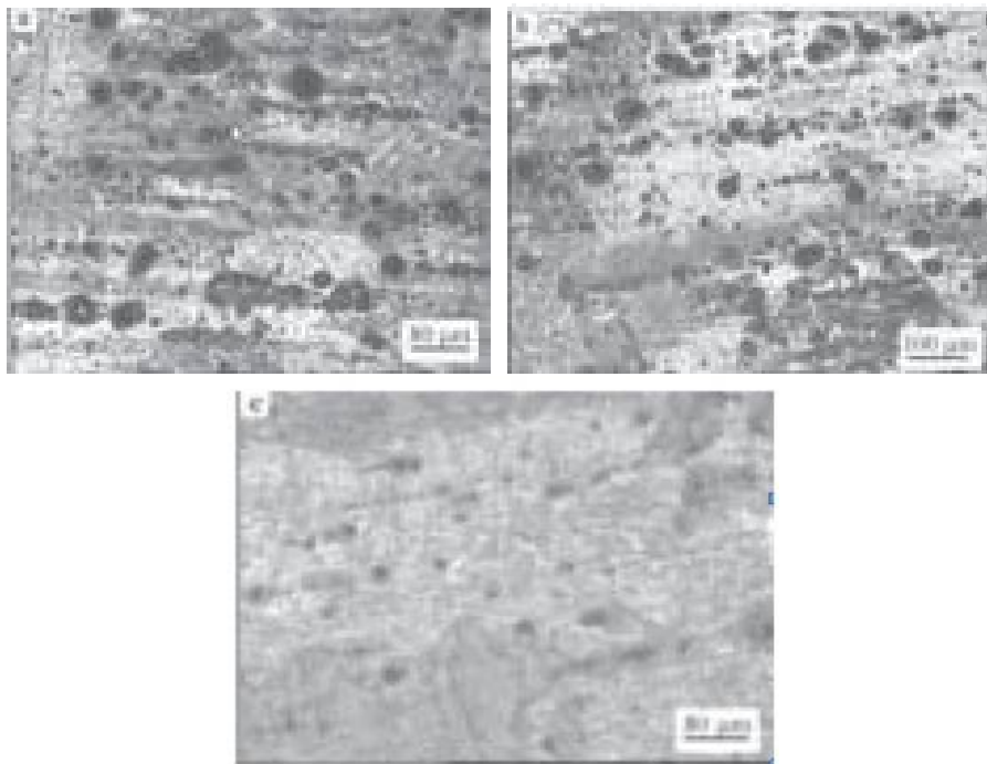
Fig.6 : Microstructures showing pits after potentiodynamic polarization in 3.5% NaCl aqueous solution (a) base metal, (b) TMAZ and (c) weld. The microstructures of pitted surfaces shown in Fig 6a-c and it reveals clearly that pit density of weld region is much less than that of base metal and TMAZ. Hence it can be concluded that pitting resistance of weld region is better than that of base metal and TMAZ. However there exists a problem of galvanic kind of corrosion because of difference in pitting potentials across the friction welded joint, especially in aggressive environments containing halide ions. Therefore corrosion protection of these welds with conversion layer coatings is highly desirable.
