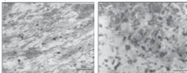
Fig. 3 : (a) Microstructure in TMAZ (b) Distribution of precipitates in TMAZ
