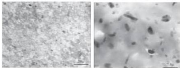
Fig. 2 : (a) Equiaxed grains in weld nugget (b) Precipitates in weld nugget
