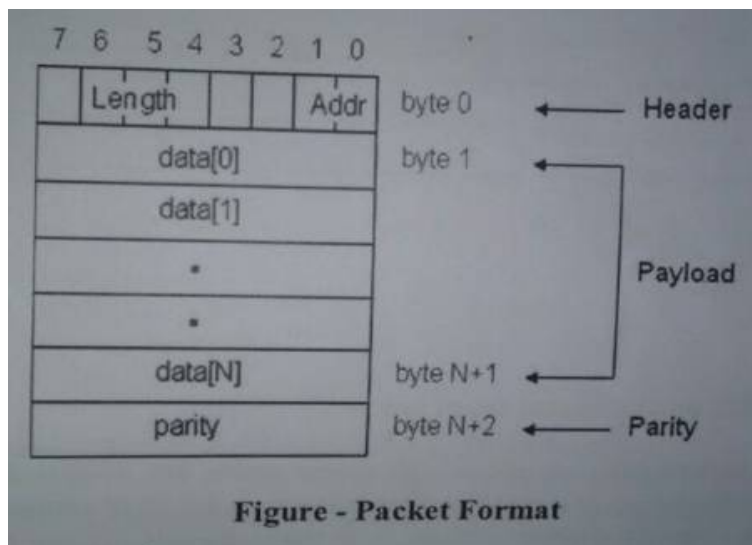
Figure 4: Packet format of a Router
