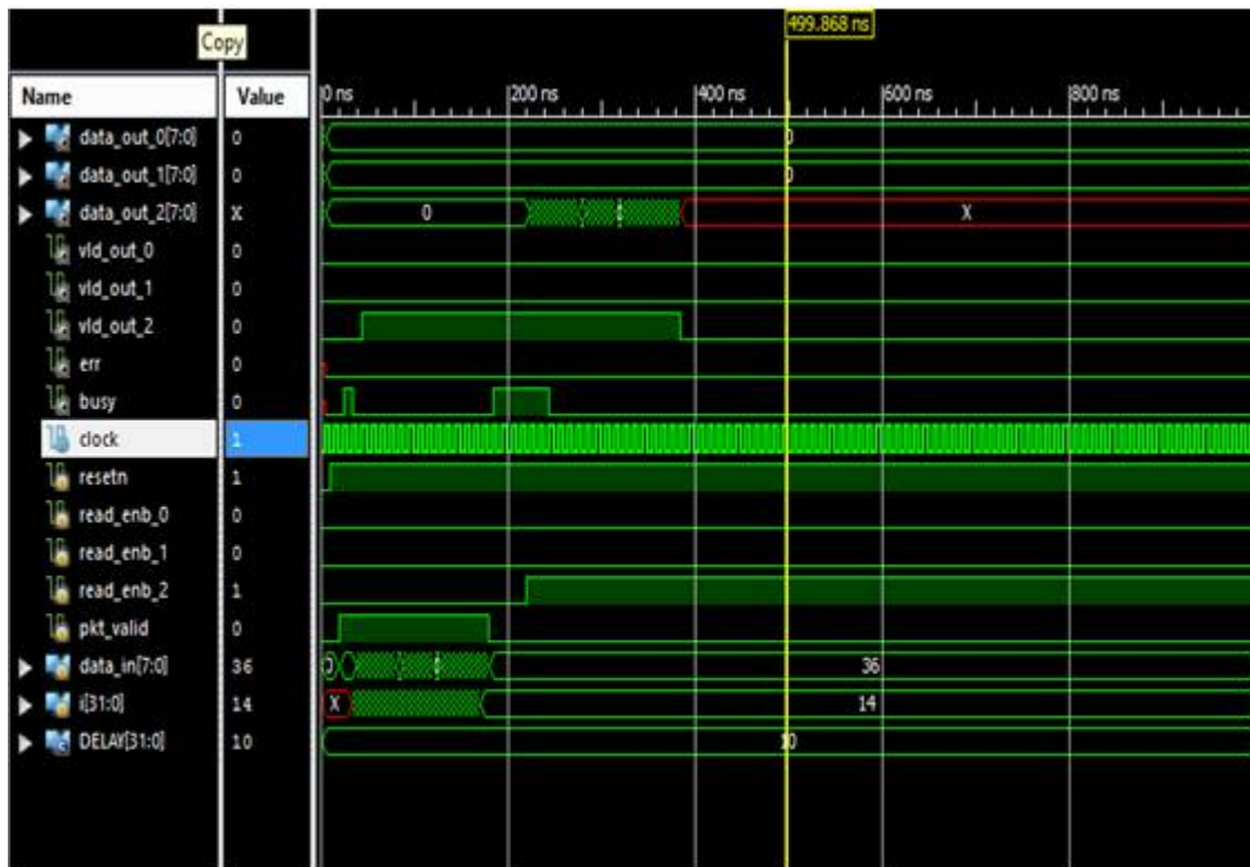
Figure 13: Top output
