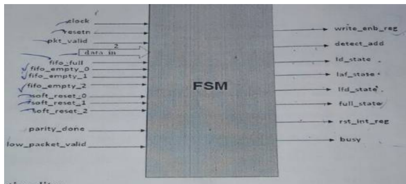
Figure 8: Router FSM
