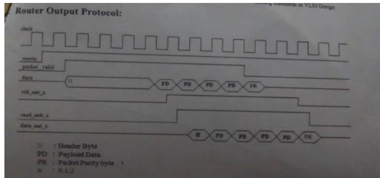
Figure 6: Router Output Protocol
