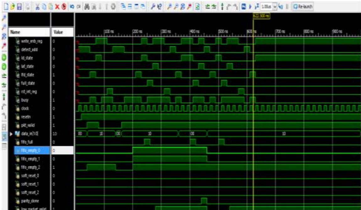
Figure 11 : Fsm output
