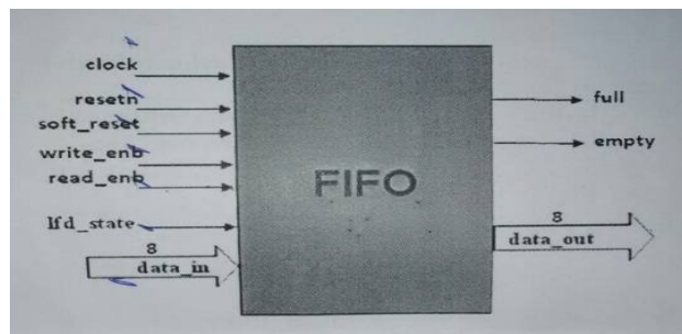
Figure 6: Router FIFO
