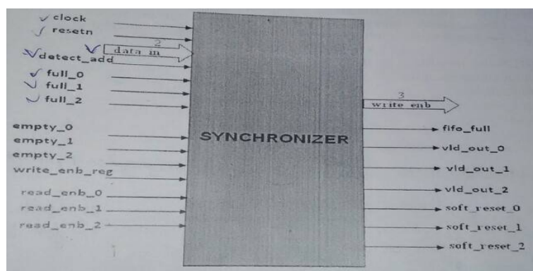
Figure 7: Router Synchronizer
