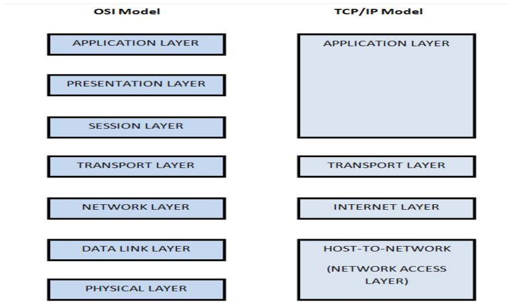
Figure 3: Diagrammatic Comparison between OSI Reference Model and TCP/IP Reference Model
