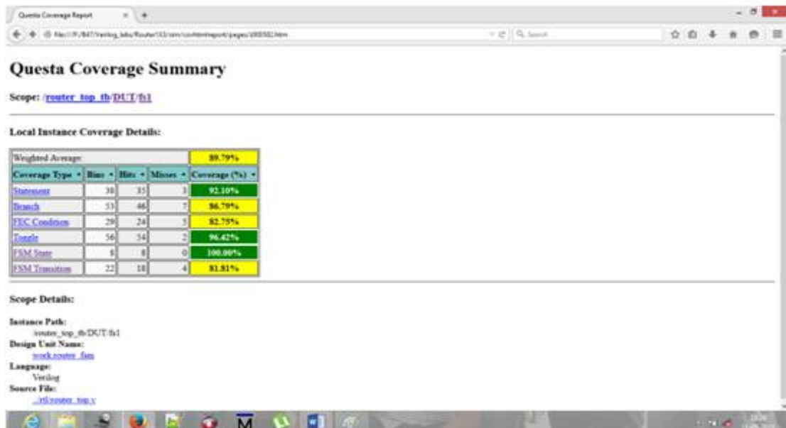
Figure 15 : Coverage Report
