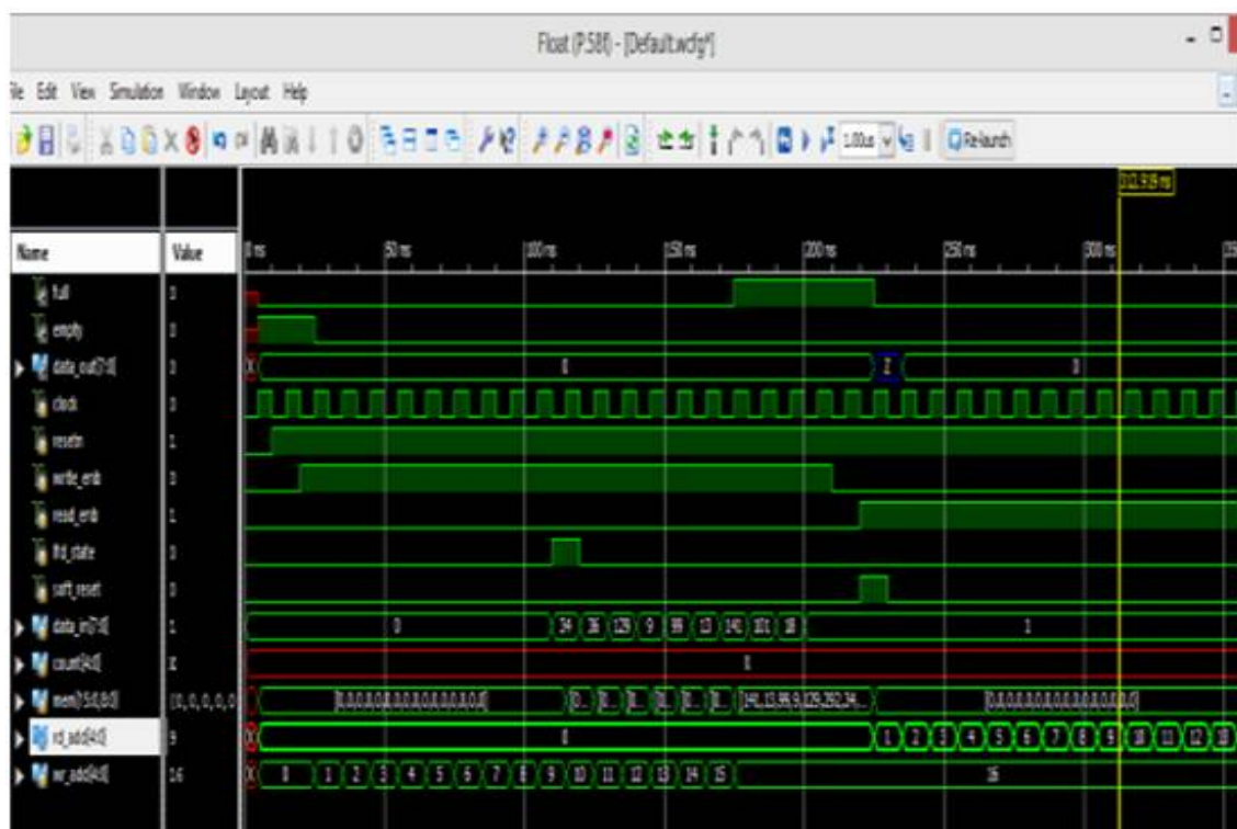
Figure 10 : Fifo output
