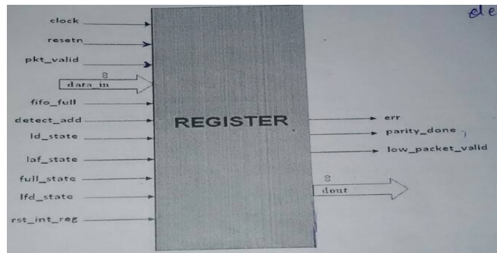
Figure 9: Router : Register
