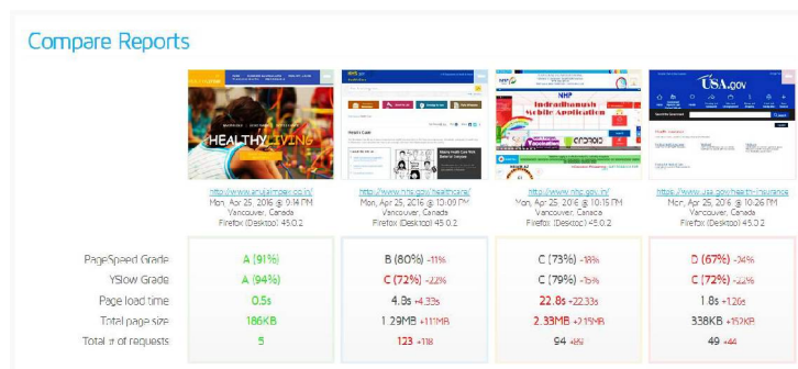
Fig 4: Comparison Report (AJAX Vs Traditional Web Applications)
