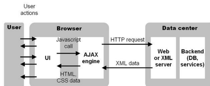
Fig 1: Generalize Architecture of Ajax.
