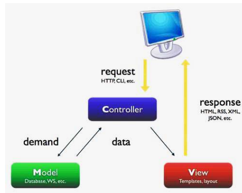
Fig 2: MVC Modeling
