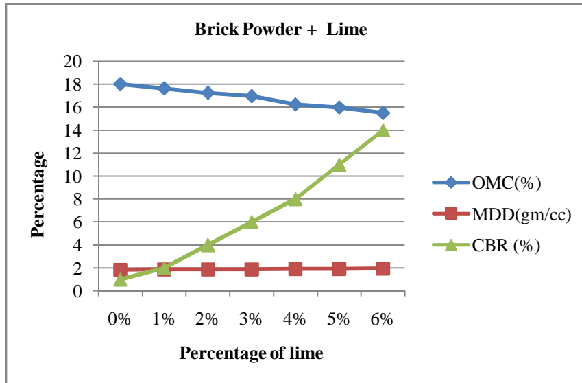
Fig. No.3. Graph Shows the Effect of Lime on OMC, MDD and CBR of Black Cotton Soil.
