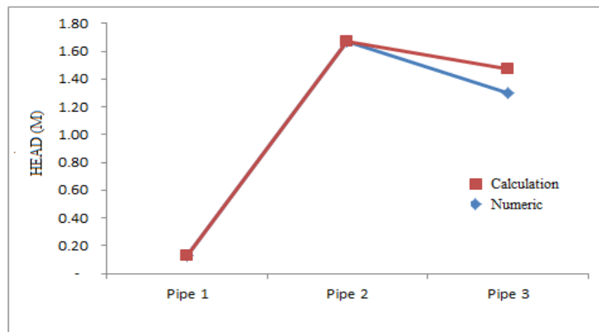
Figure 4 Comparison of manual calculations and Epanet 2.0 software
