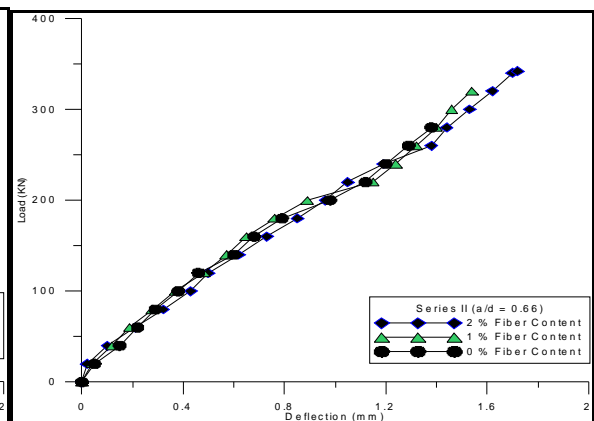
Figure IV: The graph of central deflection with respect to load, series-II
