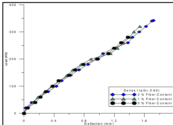
Figure III: The graph of central deflection with respect to load, series-I
