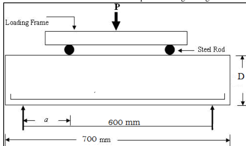
Figure I :Two point bending test set-up
