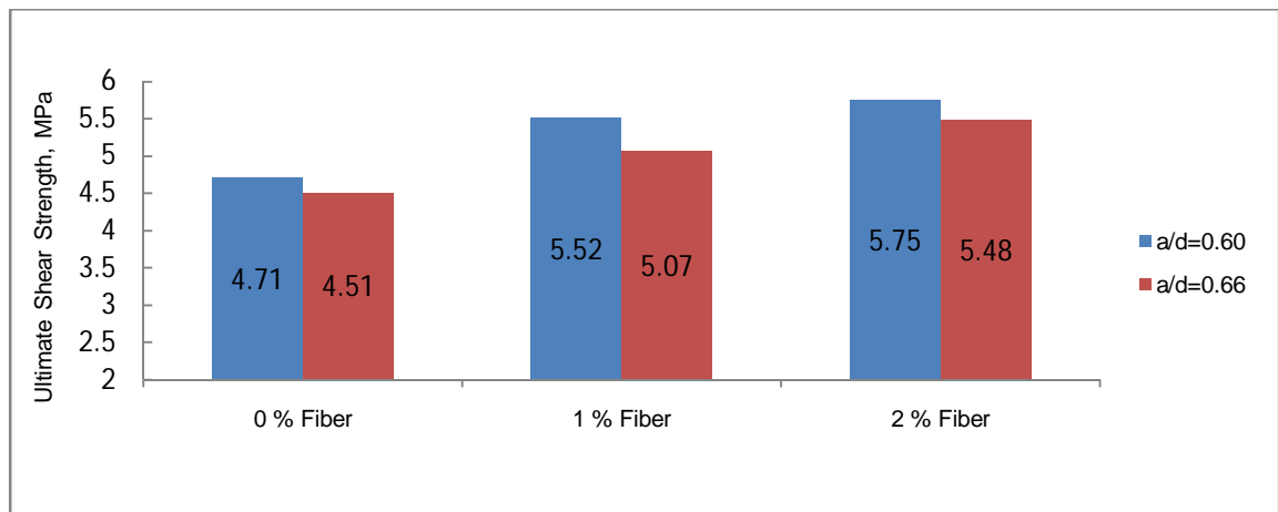
Figure II : Ultimate shear strength of beam with respect to a/d ratio and fiber content.
