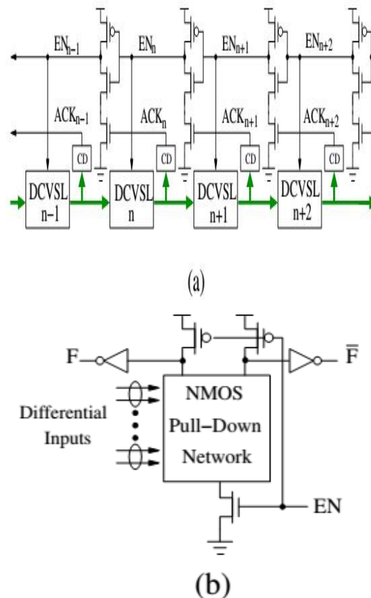
Fig. 1. (a) Zero-delay-overhead self-timed pipeline structure, and (b) DCVSL structure.
