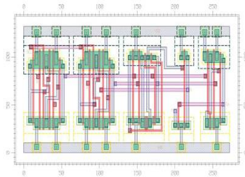
Fig. 3. CMOS implementation of PASTA. (a) Single-bit sum module. (b) 2x1 MUX for the 1 bit adder. (c) Single-bit carry module. (d) Completion signal detection circuit.
