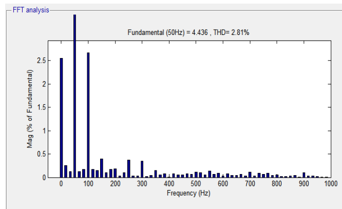
Fig. 11. Proposed PI controller-Gird Current THD =2.81%
