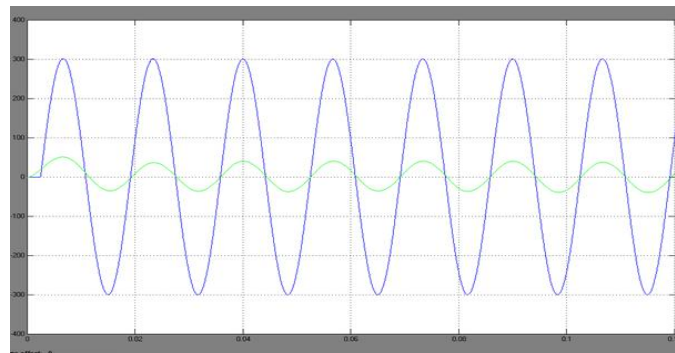
Fig. 9. Grid sharing and grid injecting modes of operation: (a) PCC voltage and grid current (phase-a).
