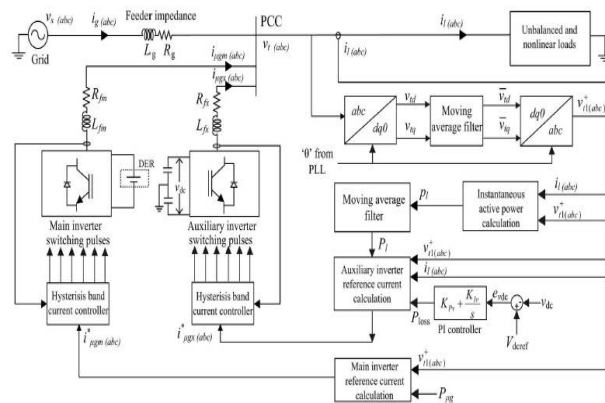
Fig. 4. Schematic diagram showing the control strategy of proposed DVSI scheme.
