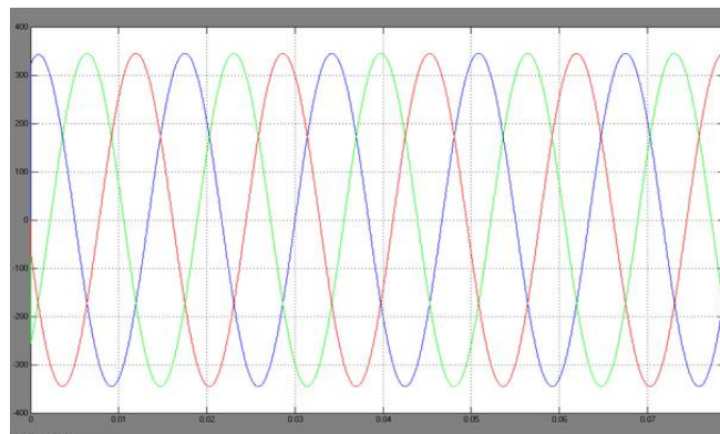
Fig. 5. Without DVSI scheme: (b) fundamental positive sequence of PCC voltages.
