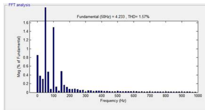
Fig. 12: With FUZZY controller-Gird Current THD = 1.57%
