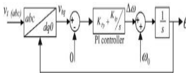
Fig. 2. Schematic diagram of PLL.
