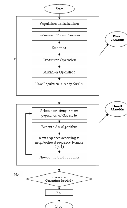
Fig 1 Flowchart for GA-SA
