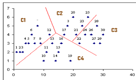
Figure 3 K-Means Clustering
