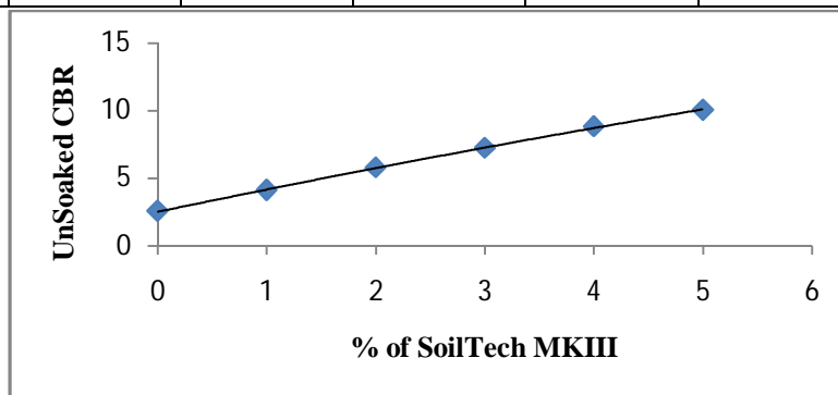
Fig 2: Variation in the Unsoaked CBR Values of Soil for Various % of SoilTech MKIII
