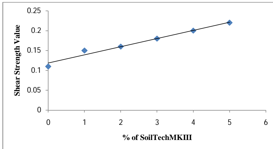
Fig 4: Variation in the Shear Strength Values of Soil for Various percentages of SoilTech MKIII
