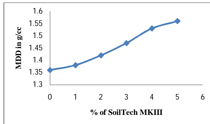
Fig 1: Variations in the MDD Values of Soil for Various % of SoilTech MKIII
