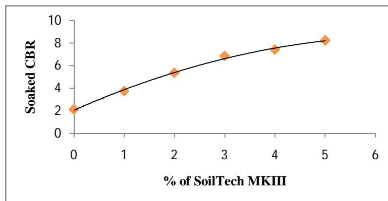
Fig 3: Variation in the Soaked CBR Values of Soil for Various Percentages of SoilTech MKIII
