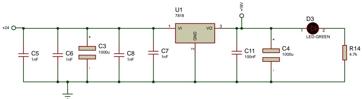
Figure 4. DC Motor Driver Power Circuit
