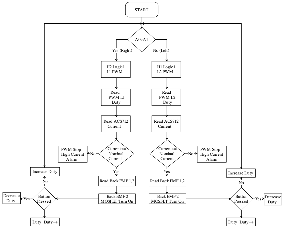
Figure 6. DC Motor Control Algorithm
