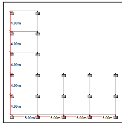
Fig. 6- L Shape (S-5)
