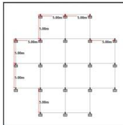
Fig. 8- Plus (+) Shape (S-7)
