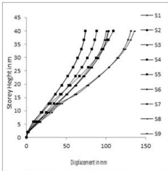
Fig.13- Storey Drift in X-Direction
