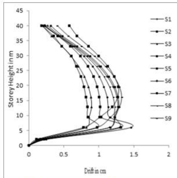
Fig.14- Storey Drift in Y-Direction
