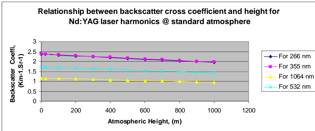
Graph (6) shows atmospheric backscatter coefficient versus height for laser wavelengths of Nd:YAG harmonics.
