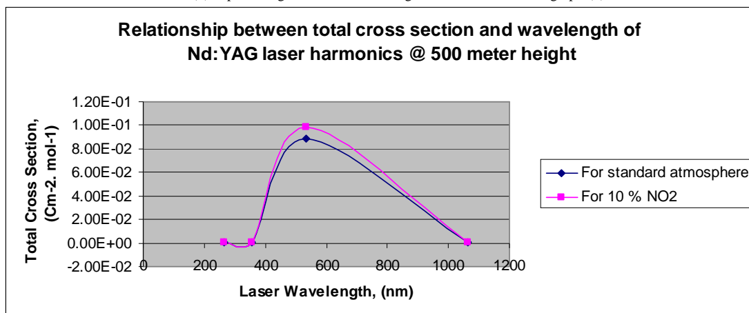
Graph (5) shows atmospheric total cross section versus wavelength of Nd:YAG laser harmonics for standard atmosphere compared with polluted atmosphere.
