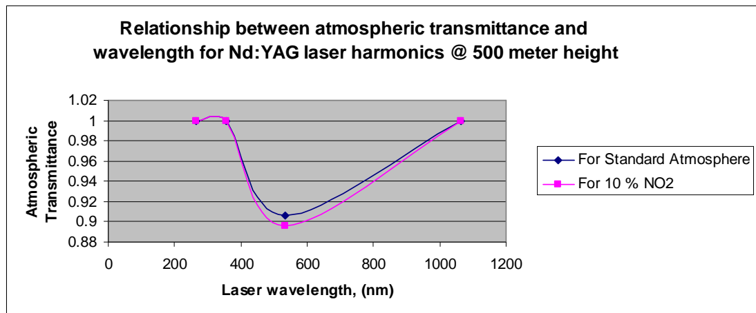
Graph (10) shows atmospheric transmittance for standard & 10 % NO 2 pollutant as a function of Nd:YAG harmonics laser wavelengths @ 500 meter height.
