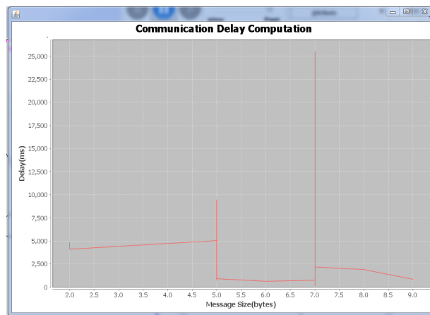
Fig. 3. Delay Computation
