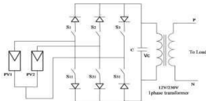
Fig.6 proposed soft switched multi string inverter
