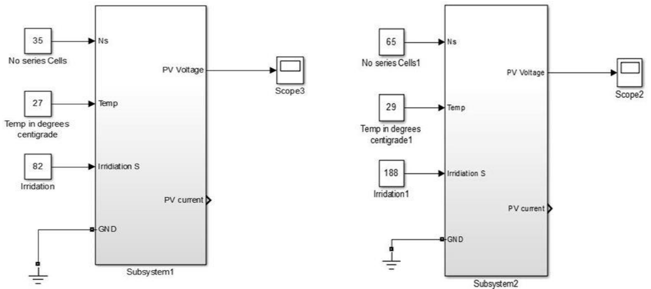
Fig.4 Solar subsystem Simulink design
