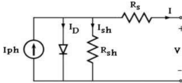
Fig. 2 PV cell equivalent circuit (Salmi et al. 2012)
