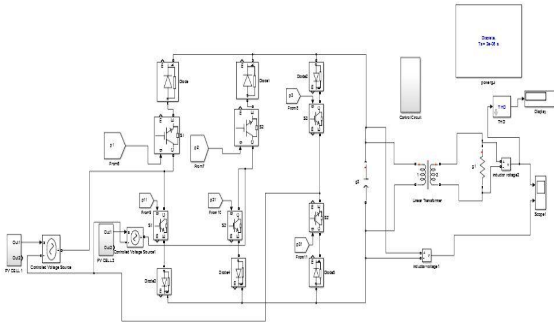
Fig. 10 Simulink design of proposed model
