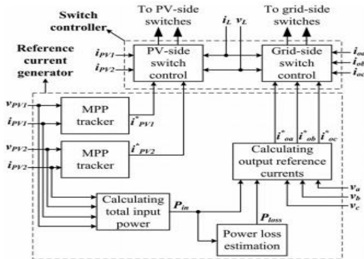
Fig 8. Control scheme of proposed multistring PV inverter
