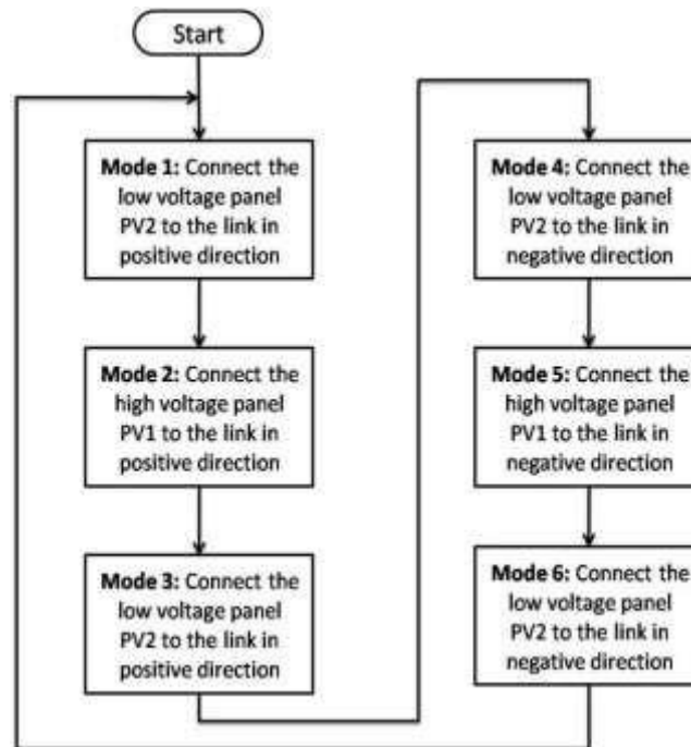
Fig. 9. Control flow chart
