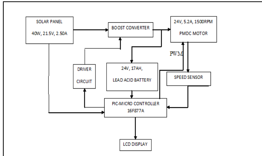
Fig 3.1: Block diagram of solar PV fed DC motor speed control system
