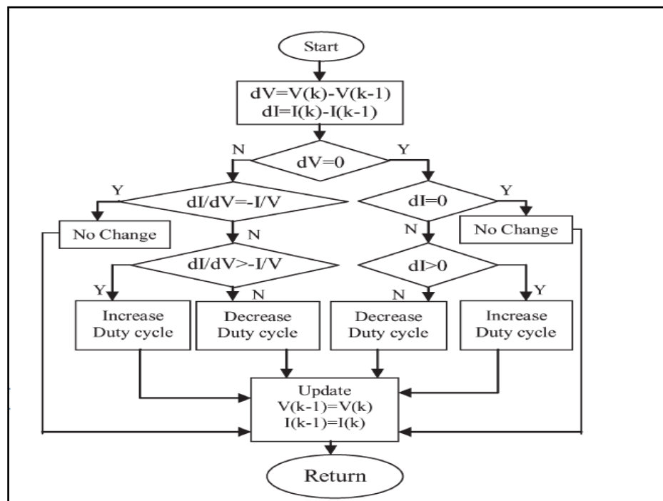
Fig 2.2: flowchart of incremental conductance algorithm
