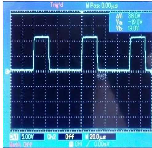
Fig 5.6: Duty cycle of boost converter at time 1.30PM
