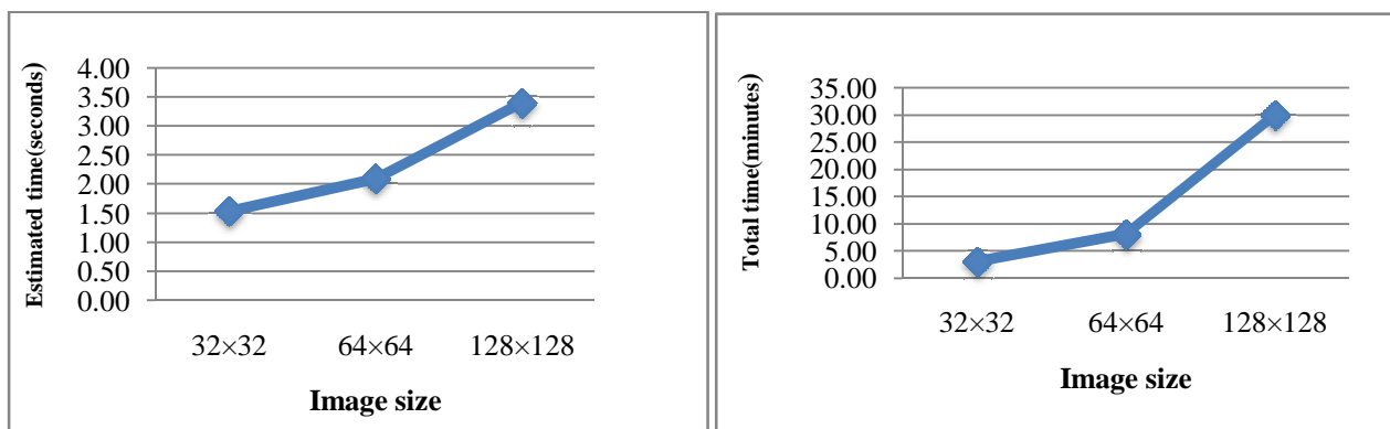
Figure 6: graph indicating different estimated times and total time for execution according to different sizes of images
