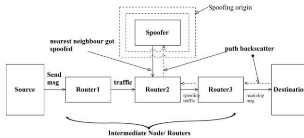
Fig. 1. Architecture of proposed work
