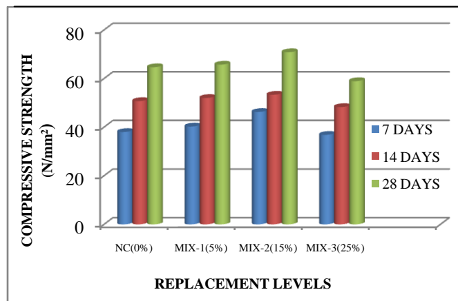
Fig No: 3 Testing of cube
