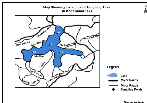
Fig 2: Sampling locations
