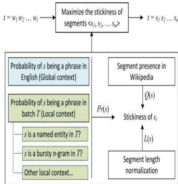
Fig 3 HybridSeg framework.
