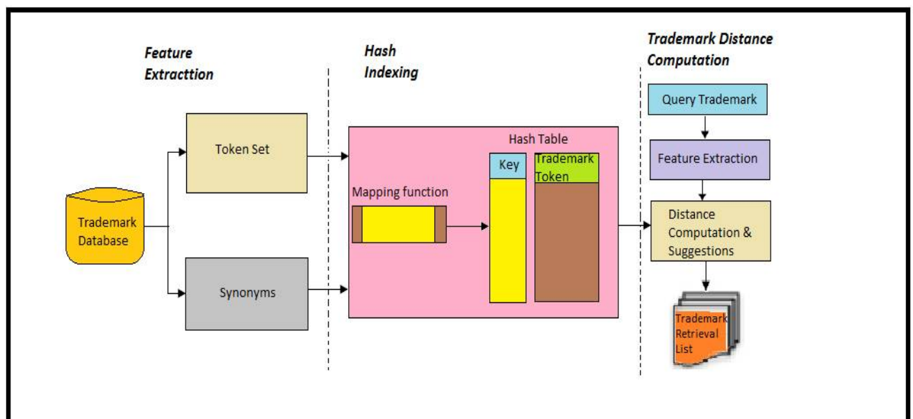
Fig. 1: Trademark System Architecture
