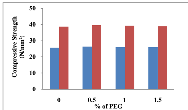
Fig. 1 Comparison of Compressive Strength
