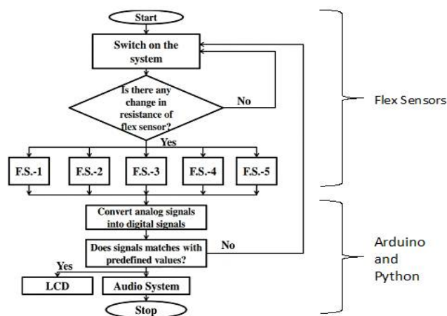
Fig. 4 System Architecture
