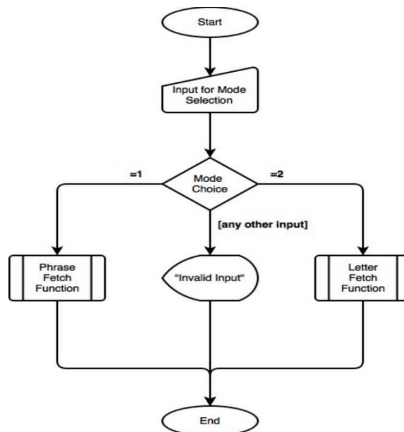
Fig. 6 System Flowchart
